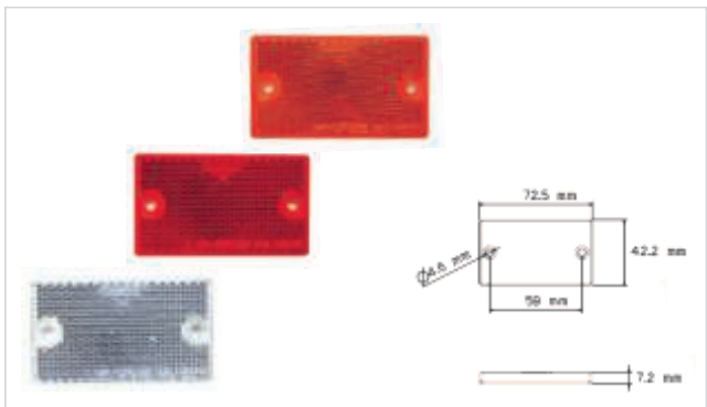
Large Surface Mount Reflex Reflector
