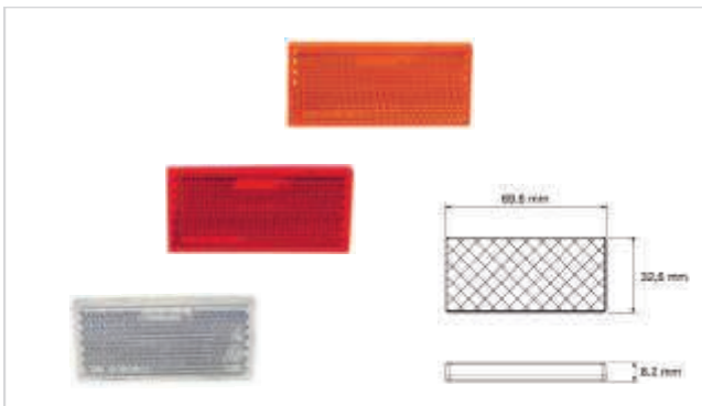
Small Surface Mount Reflex Reflector
